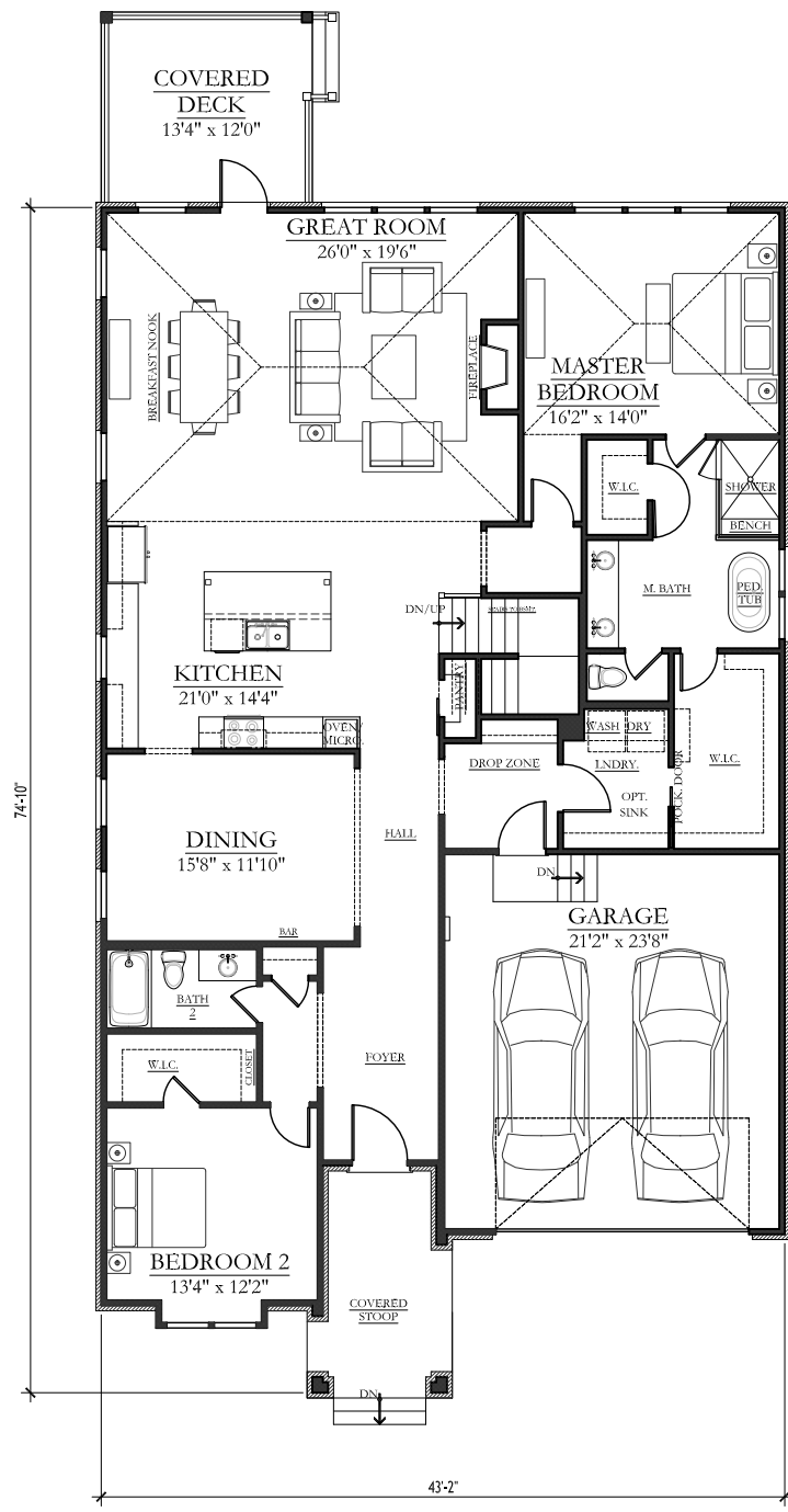
FIRST FLOOR
