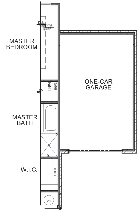
OPT. CARRIAGE GARAGE FLOOR PLAN
