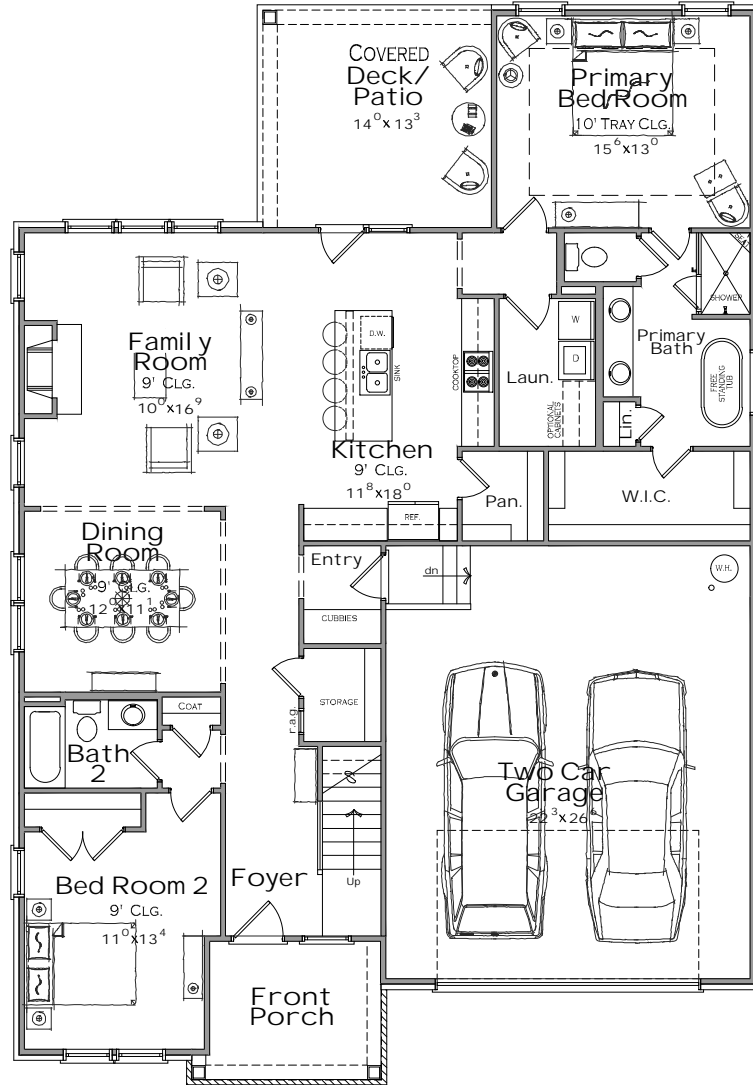
First Floor
