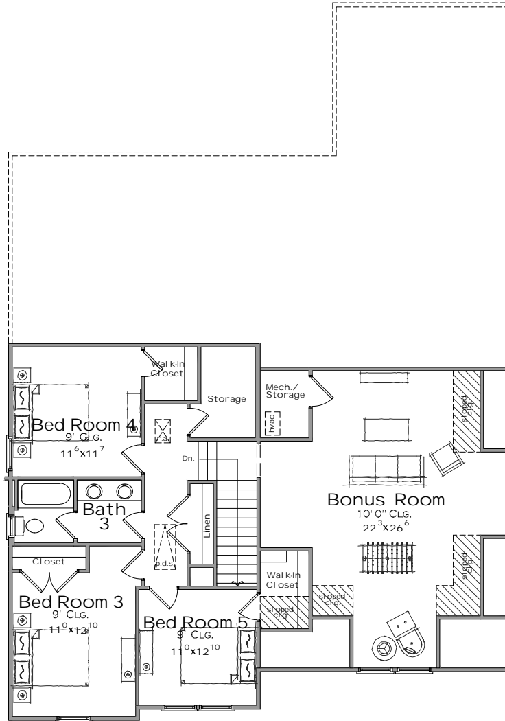
Second Floor
